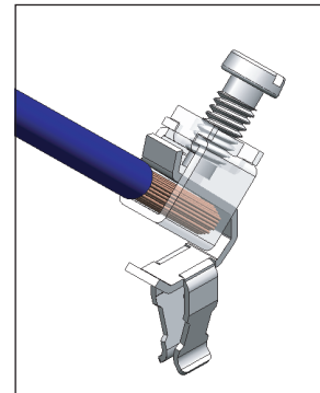
135° wire entry
